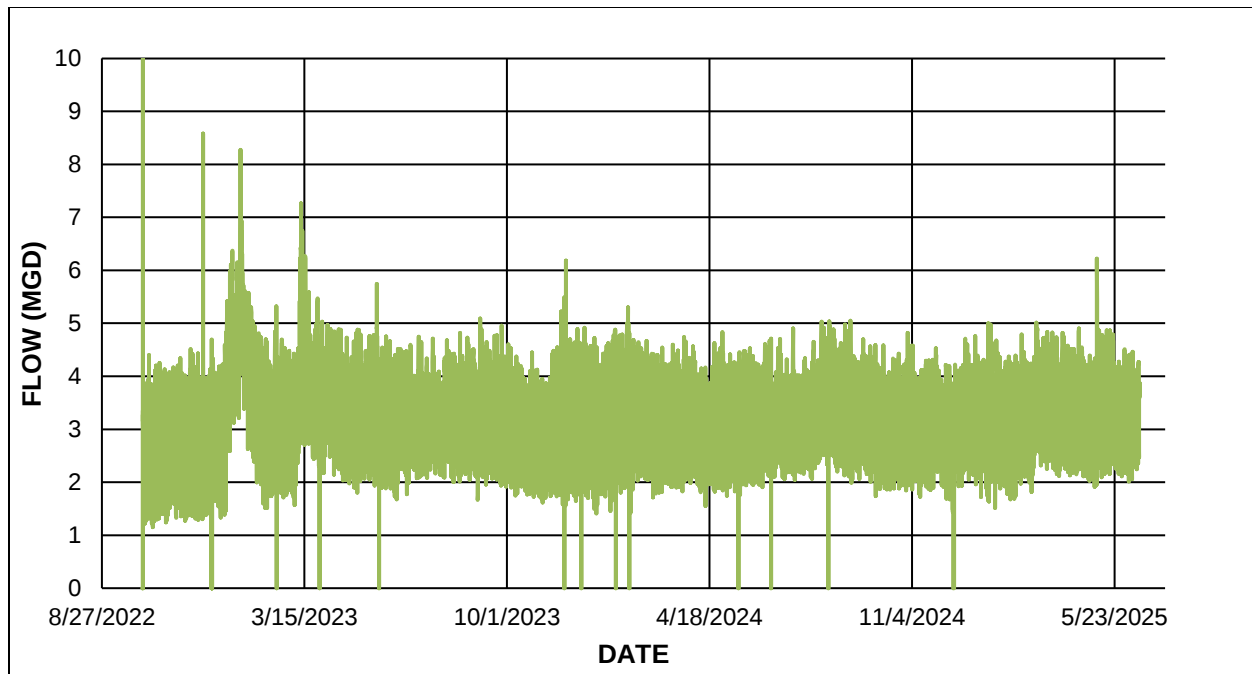
FIGURE 4-5 WRF HEADWORKS FLOW (NO PRE-TREATMENT)
