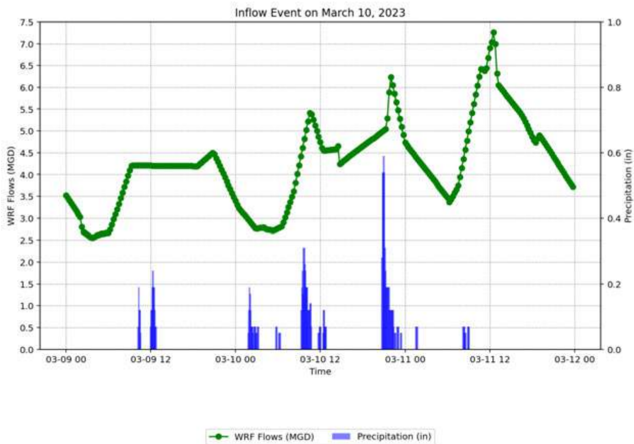
FIGURE 4-6 WRF FLOW VS. PRECIPITATION
