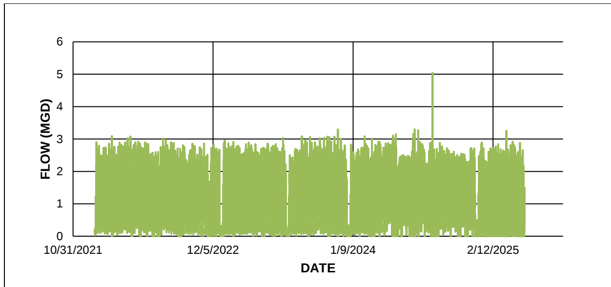
FIGURE 4-4 NESTLE PRE-TREATMENT FLOWS
