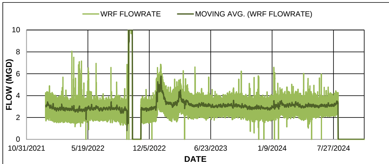
FIGURE 4-3 WRF HEADWORKS FLOW INCLUDING PRE-TREATMENT
